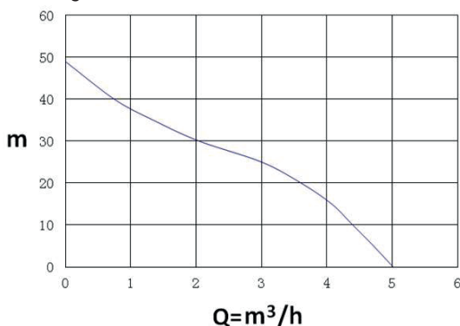
Flowdiagram
